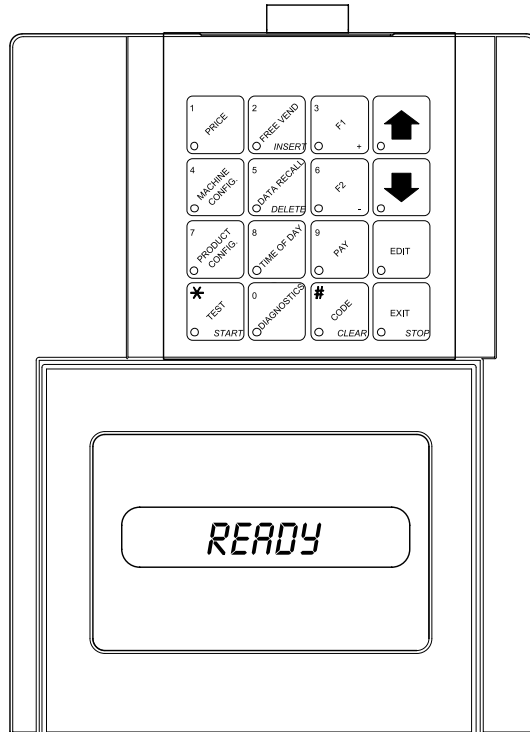
Control Panel and Display Panel (view with monetary door open)
